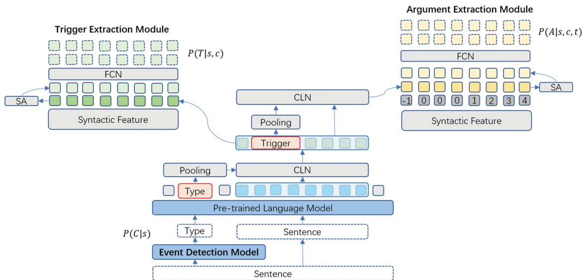
Figure 2. The overall framework of the financial event extraction approach.
